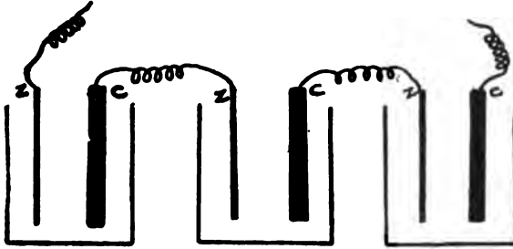
FIG. 422.—Diagram of a Series Circuit, showing Three Galvanic Cells in Battery. As shown, the copper, or positive, pole of the first cell is connected to the zinc, or negative pole of the second, and so on; leaving a negative terminal at one end and a positive at the other. Thus the current emerging from each cell passes through all those succeeding in line, the total voltage of the battery being equivalent to the sum of the individual voltages of the several cells. If, on the other hand, several motors, or other electrically affected apparatus, be connected in series, the result is to increase the "back-pressure" (C. E. M. F.) on the same ratio, and hence cut down the operative efficiency of each.
